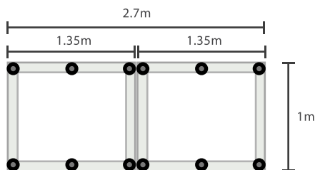
1 m x 2.7 m MODULE 12 LEGS (Two 1.35 m sections for greater layout flexibility.)
