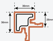
CROSSROAD TRIM
