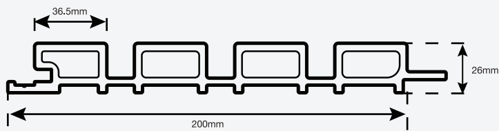
CLADDING BOARD
