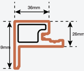
STARTER TRIM
